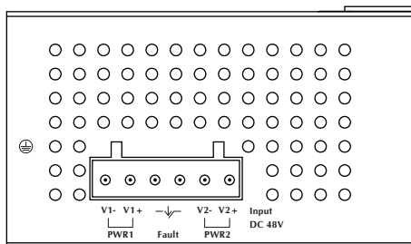
Figure 2-2 PoE Industrial Ethernet Extender Upper Panel.
