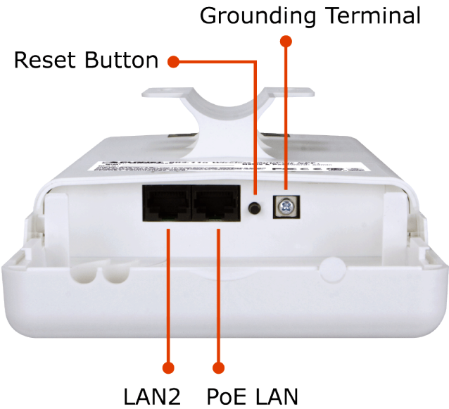
Figure 2-3 Bottom Panel
