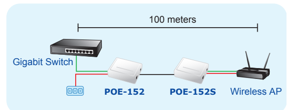
Figure 2: Connection architecture over POE-152/152S
