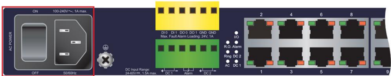
Figure 2-1-4-1: IEGS5210T-24G4GF-10G AC inlet power socket
