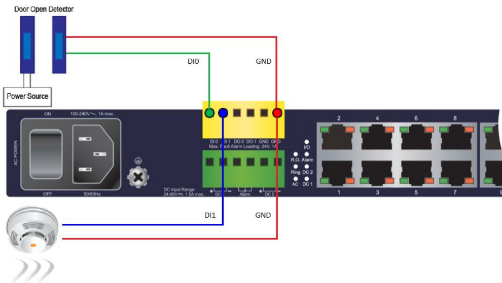
Figure 2-1-7-3 Wiring DI0 and DI1 to Open Detector
