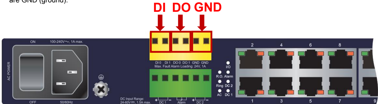
Figure 2-1-7-1a Wiring Digital Inputs/Outputs of IEGS5210T-24G4GF-10G
