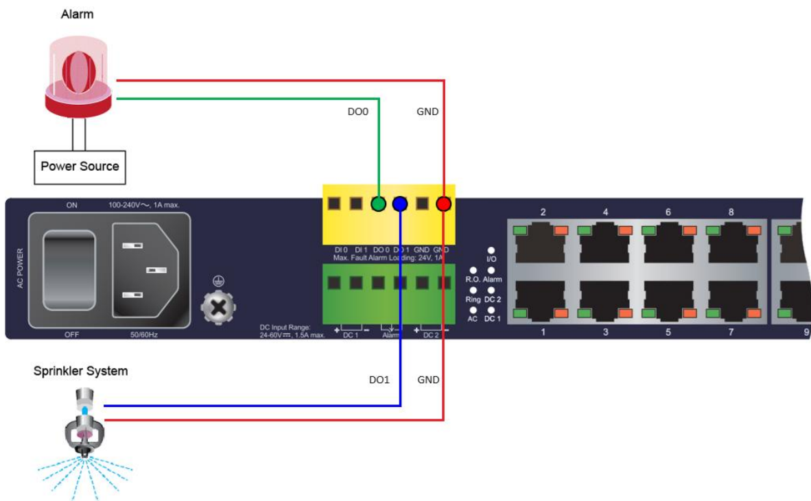
Figure 2-1-7-4 Wiring DO0 and DO1 to Open Detector
