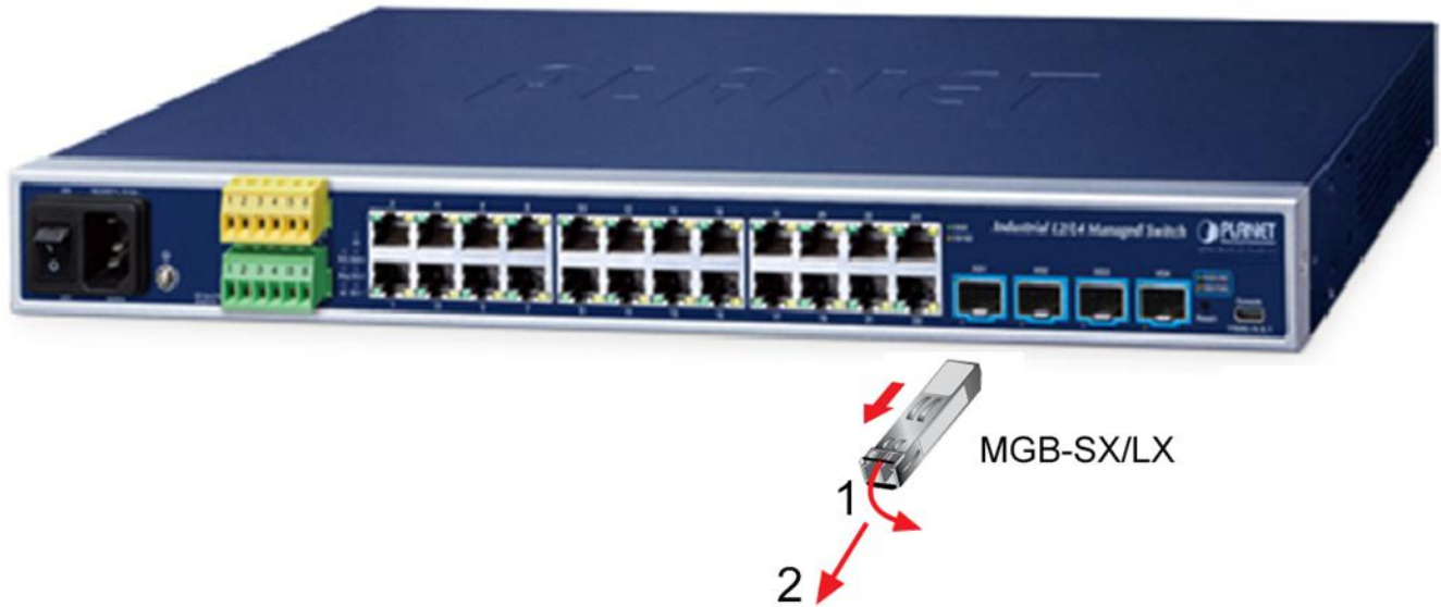
Figure 2-3-2-1: Pull out the SFP Transceiver Module
