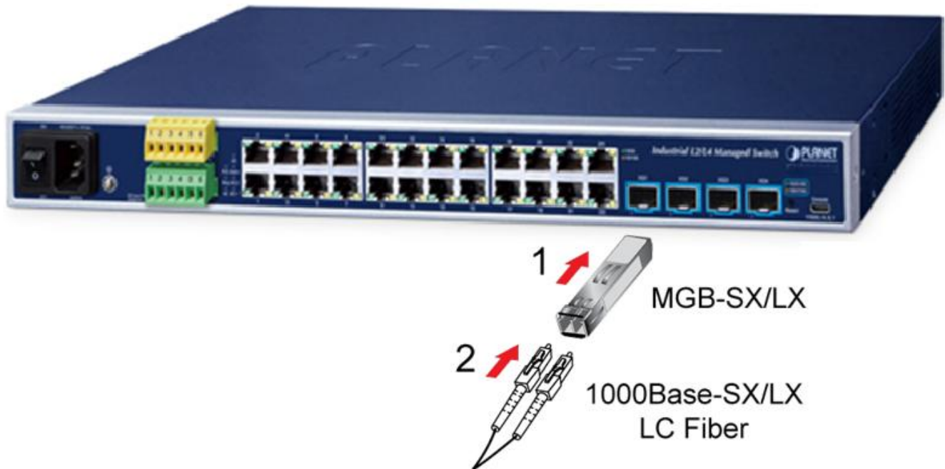
Figure 2-3-1-1: Plug in the SFP/SFP+ Transceiver
