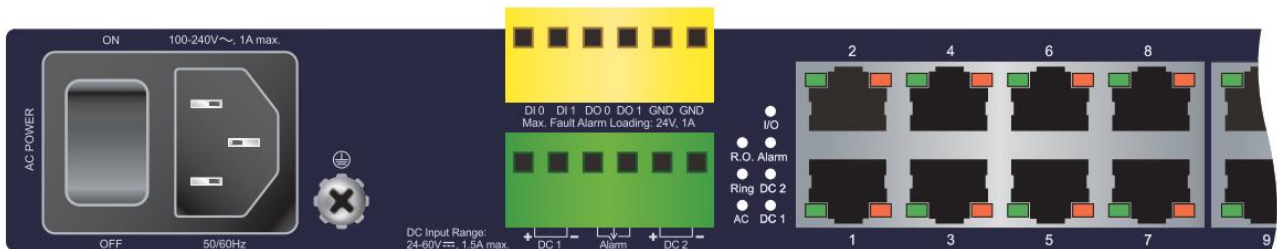
Figure 2-1-3-1a: IEGS5210T-24G4GF-10G LEDs on Front Panel
