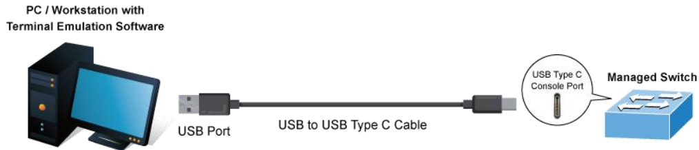
Figure 3-3-1: Console Management
