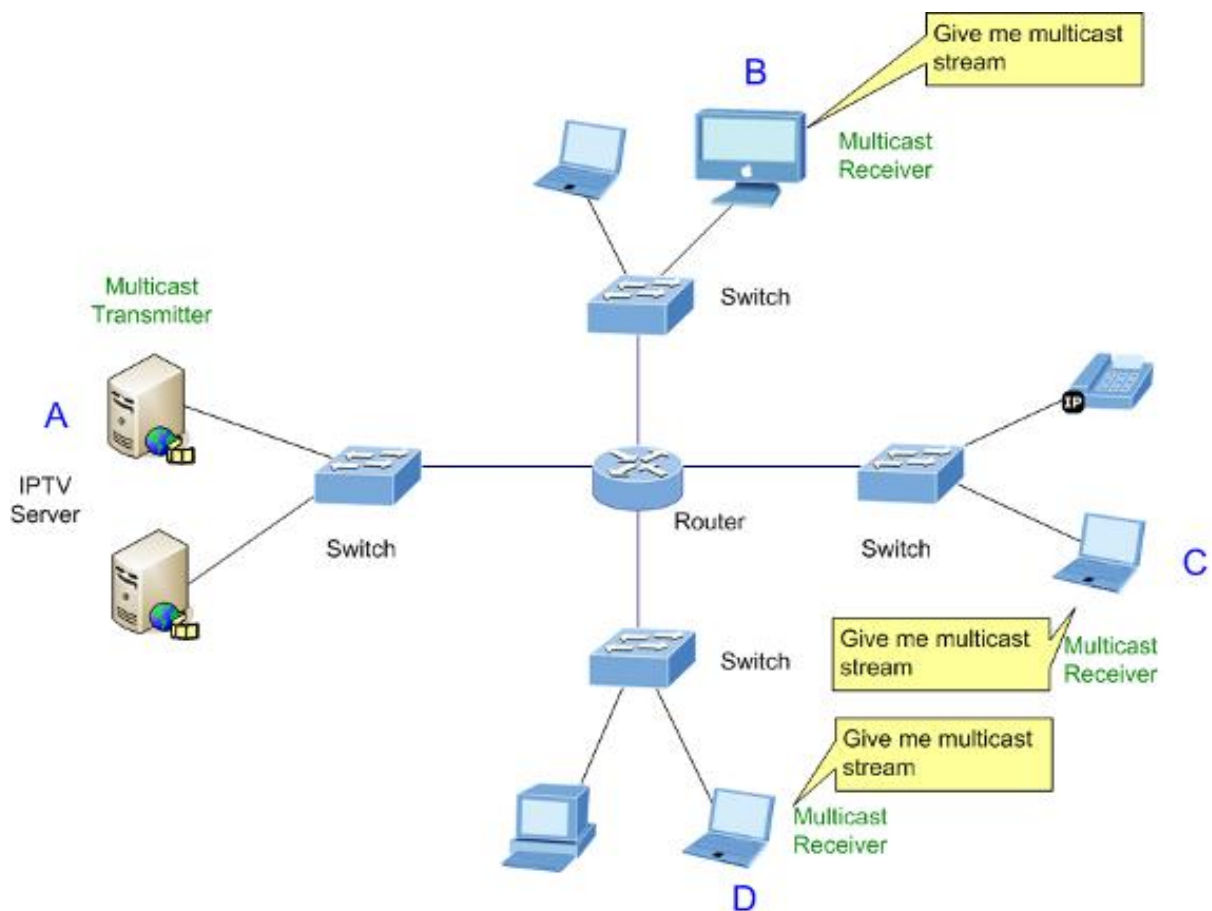
Figure 4-8-1: Multicast Service
