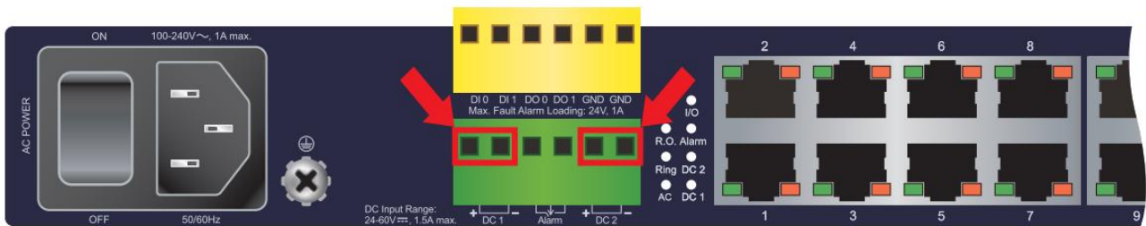
Figure 2-1-5-1: IEGS5210T-24G4GF-10G DC power input
