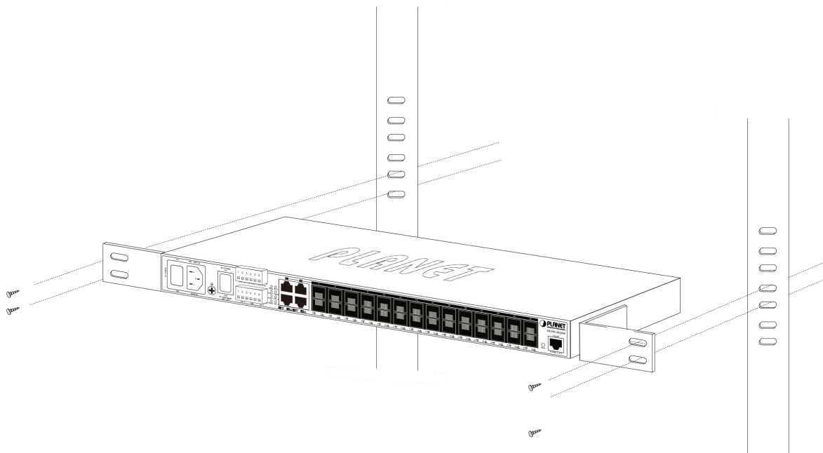
Figure 2-2-2-1 Mounting the Industrial Managed Switch on a Rack
