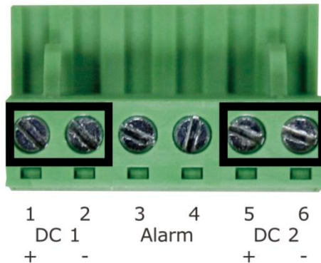
Figure 2-1-5-2 6-pin Terminal Block Power Wiring Input for IEGS5210T-24G4GF-10G
