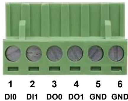
Figure 2-1-7-2 6-pin Terminal Block for DI and DO Wiring Input
