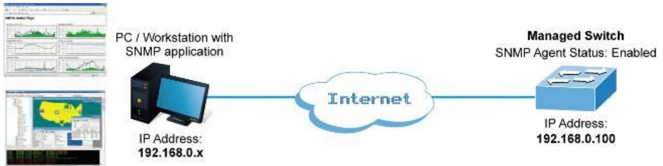
Figure 3-5-1: SNMP Management
