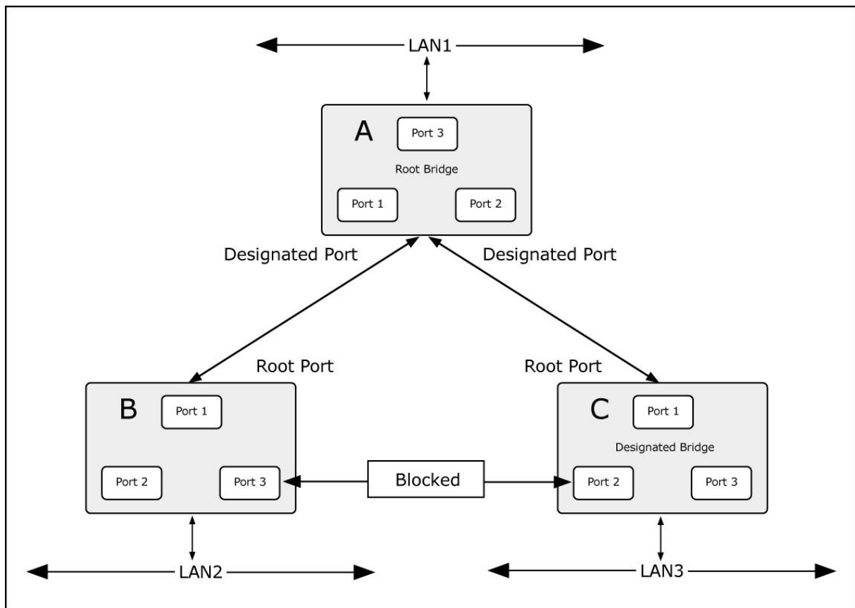
Figure 4-6-1-2: After Applying the STA Rules
