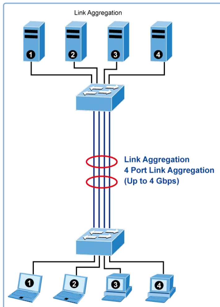
Figure 4-4-1: Link Aggregation
